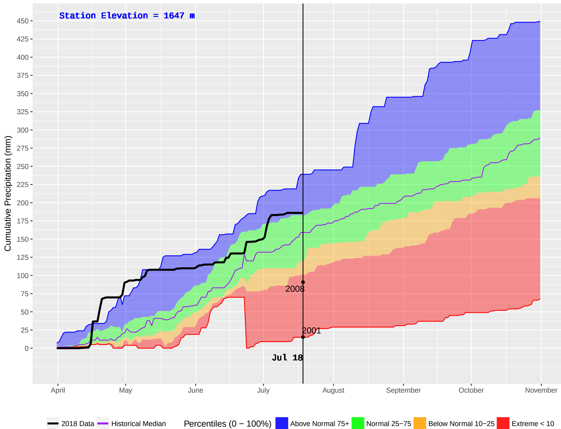
ROUND PRAIRIE (788) : Historical (2001–2016) and Current (2018) Daily Cumulative Precipitation
