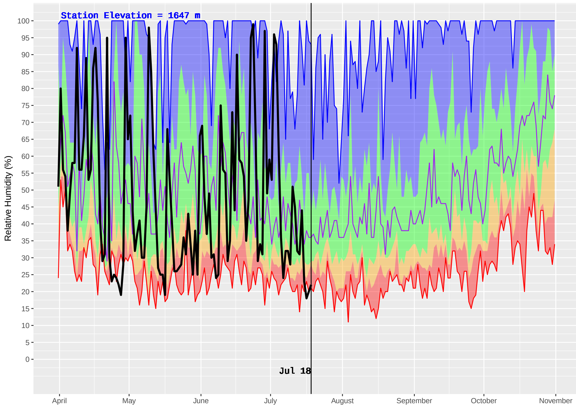
ROUND PRAIRIE (788) : Historical (2001–2016) and Current (2018) Daily Relative Humidity
