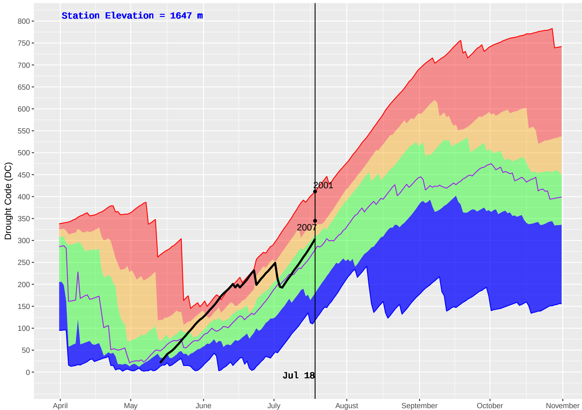
ROUND PRAIRIE (788) : Historical (2001–2016) and Current (2018) Daily Drought Code (DC)
